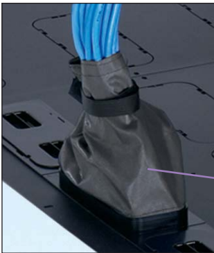
Cool Boot® Cabinet Top Air Sealing Fitting is used to seal copper data cables entering the cabinet.
