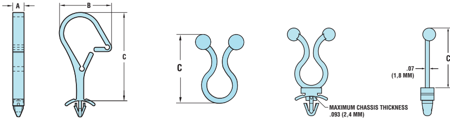
“P” Style Wire and Cable Holder
